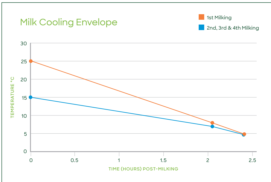
GRAPH 1 - MILK COOLING ENVELOPE
